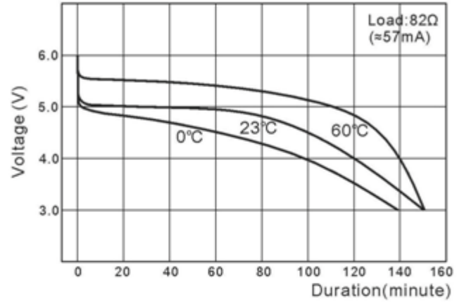
Discharge curve at various temperatures
