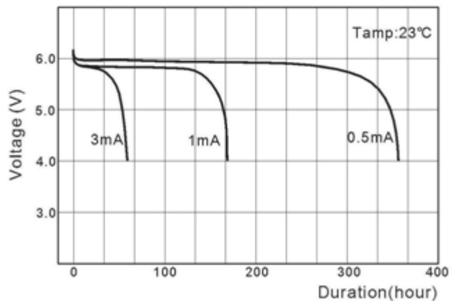
Discharge curve at various currents
